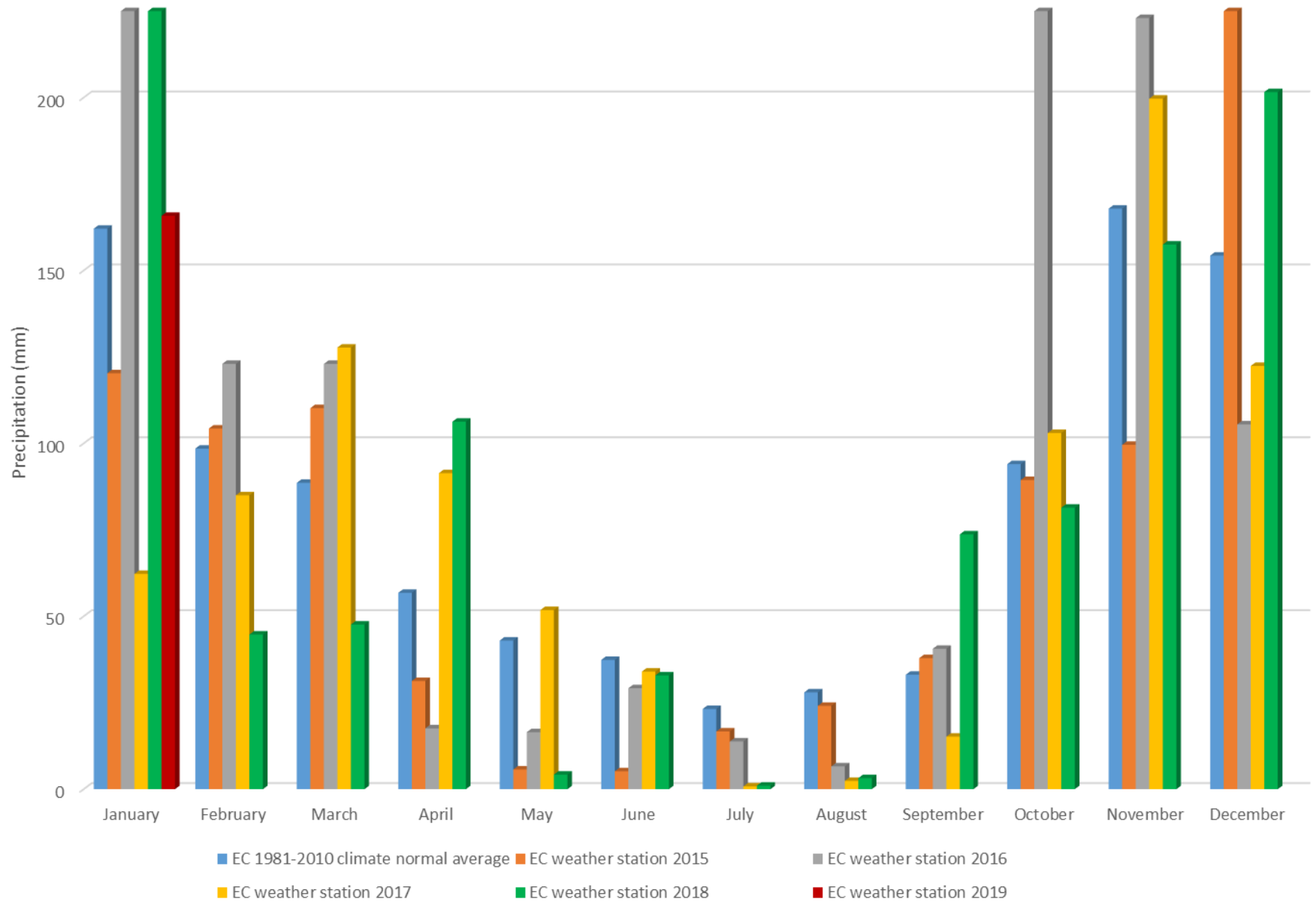
St. Mary Lake Precipitation- Updated to January 23, 2019
